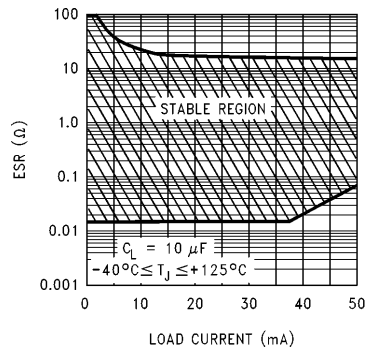
FIGURE 3. 10 \mu\text{F} ESR Range
